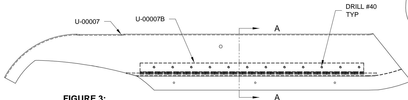
FIGURE 3: POSITIONING HINGE IN FAIRING
