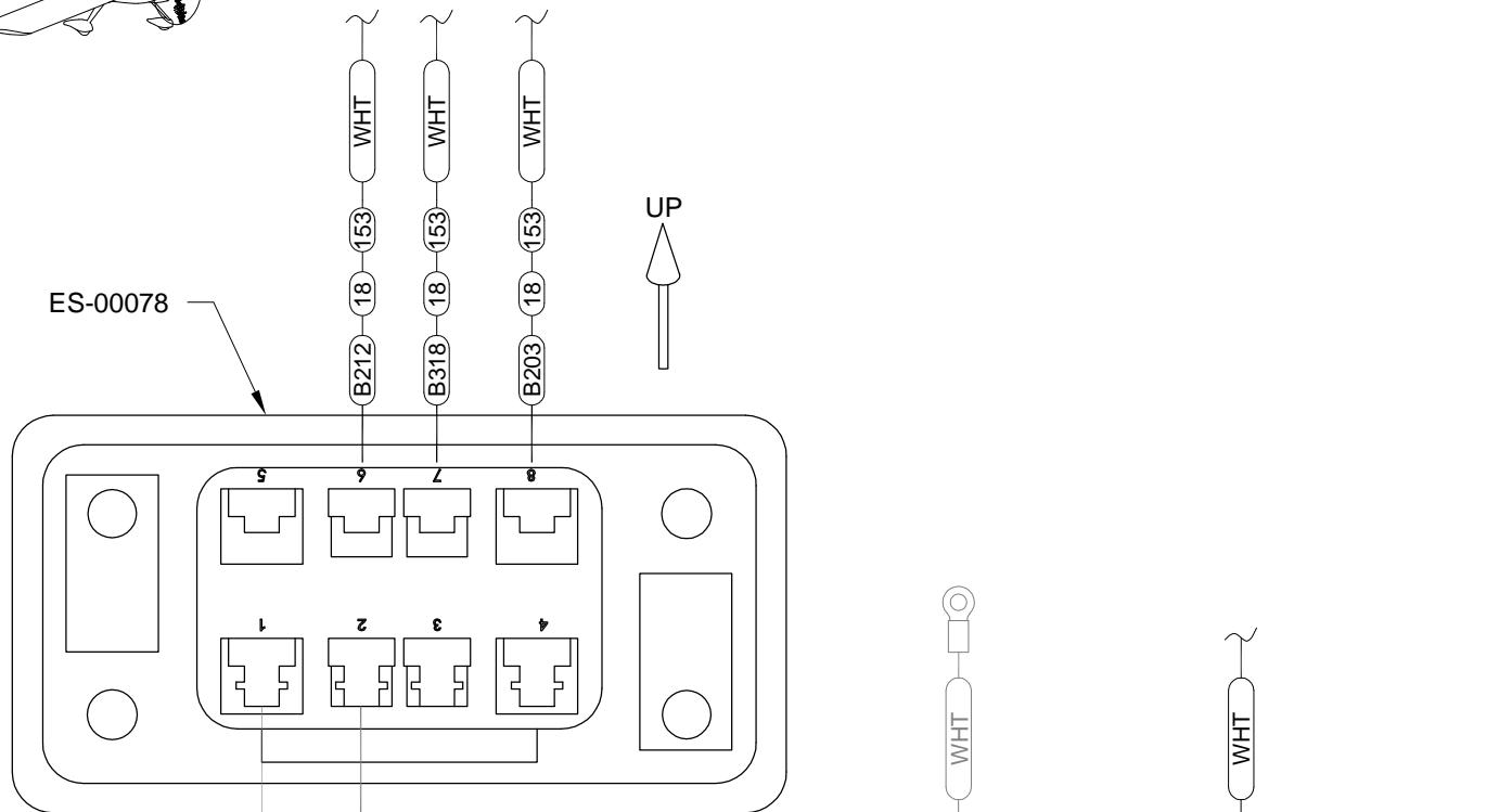
FIGURE 1: LEFT WING CONNECTOR MALE BACK VIEW
