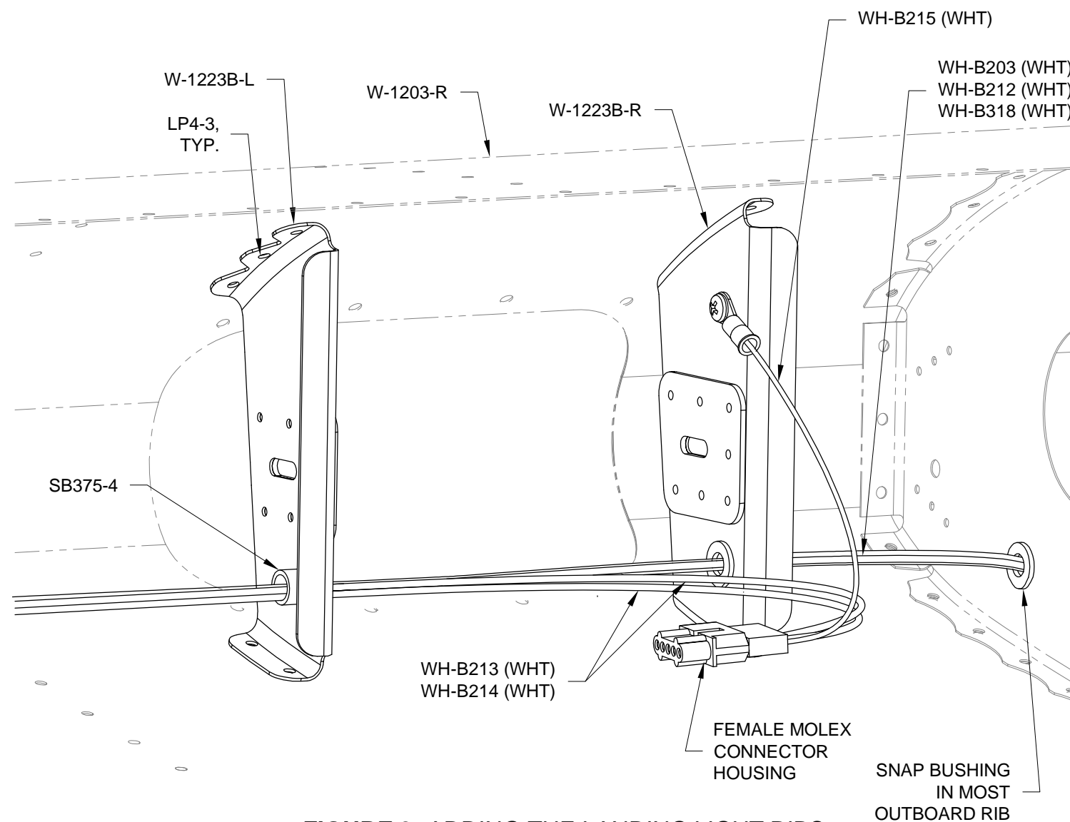
FIGURE 3: ADDING THE LANDING LIGHT RIBS (VIEW FROM INSIDE THE WING)
