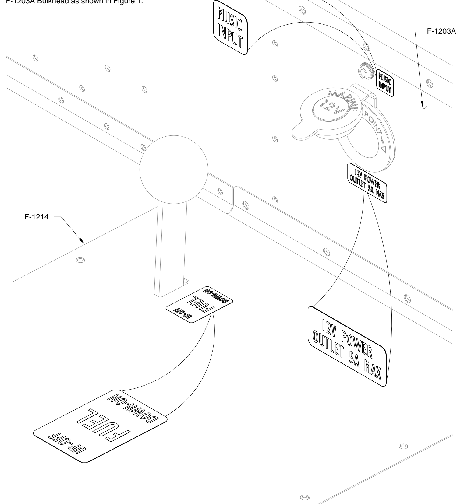
FIGURE 1: FUEL VALVE LABEL PLACEMENT
