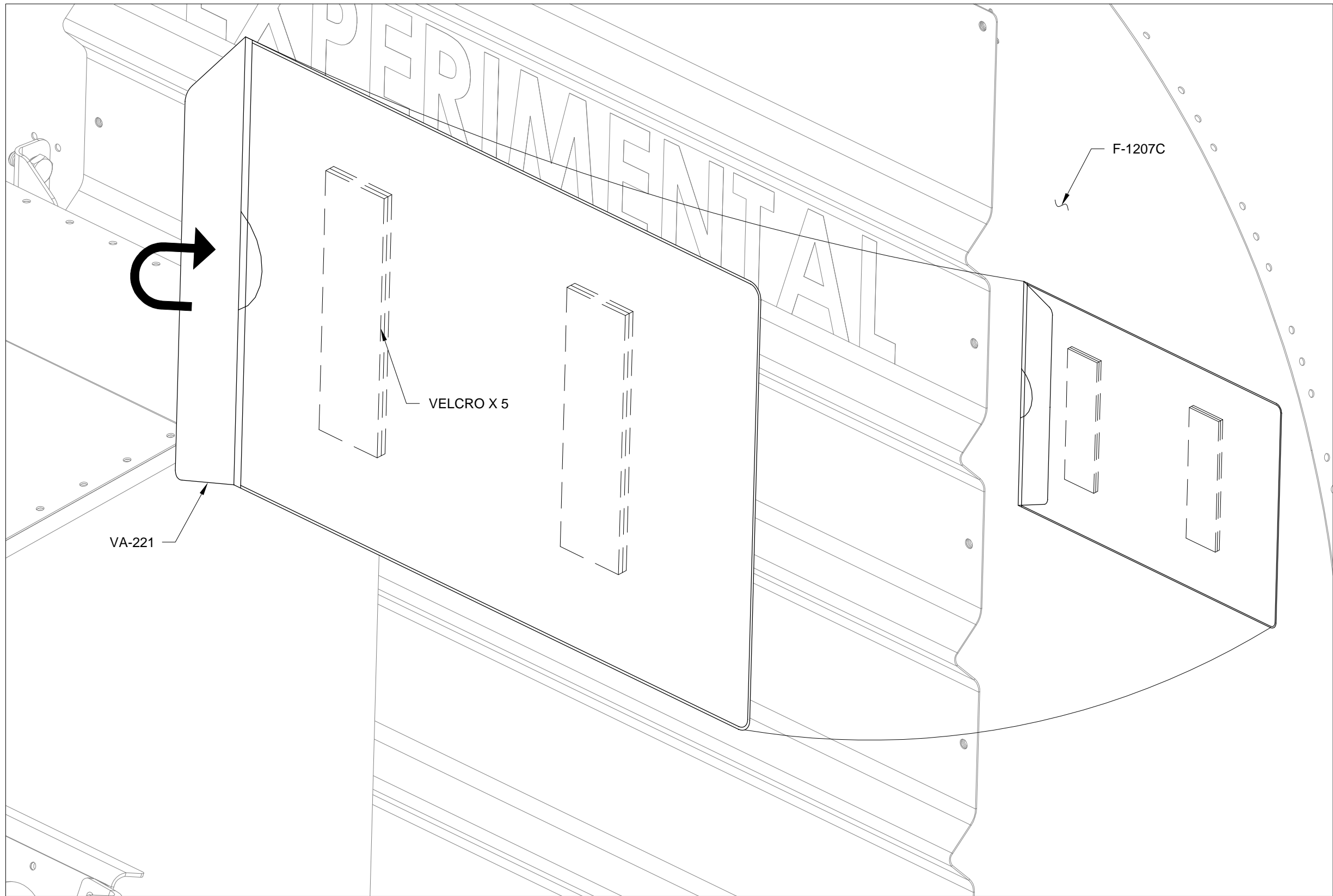
FIGURE 1: VINYL ENVELOPE PLACEMENT
