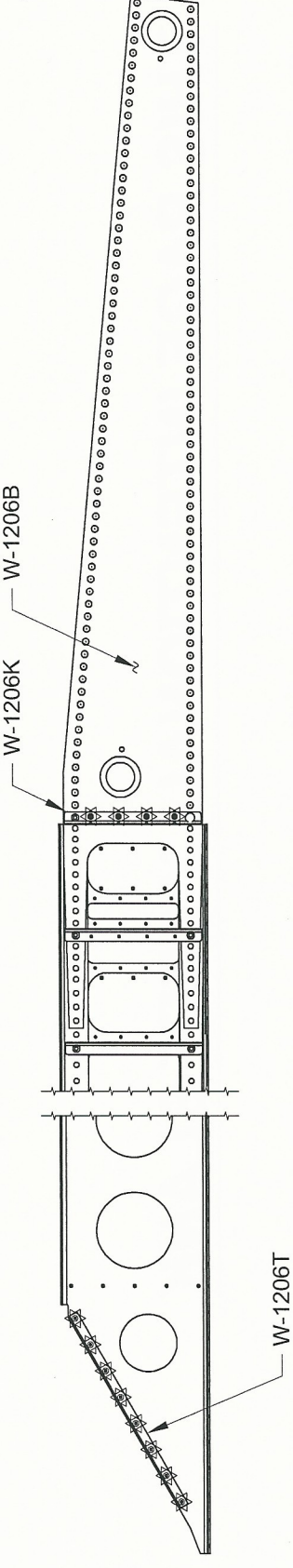
FIGURE 2: W-1206-R SPAR ASSEMBLY RIVETS
